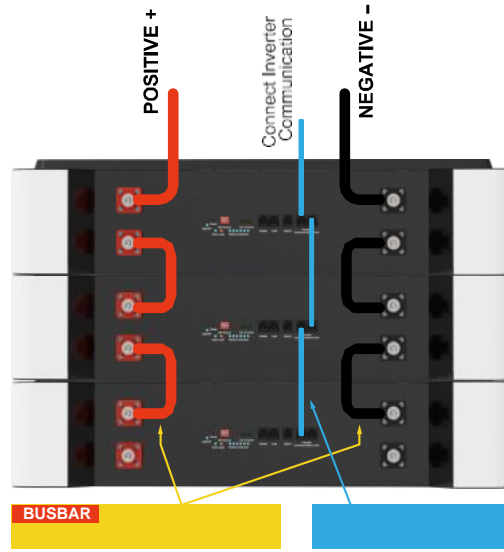
Schematic Diagram of Connection and Use of Three Batteries
