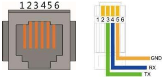
RS232 Communication Port Definition
