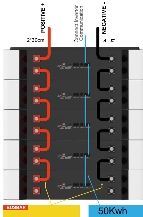
Schematic Diagram of Connection and Use of Five Batteries.
