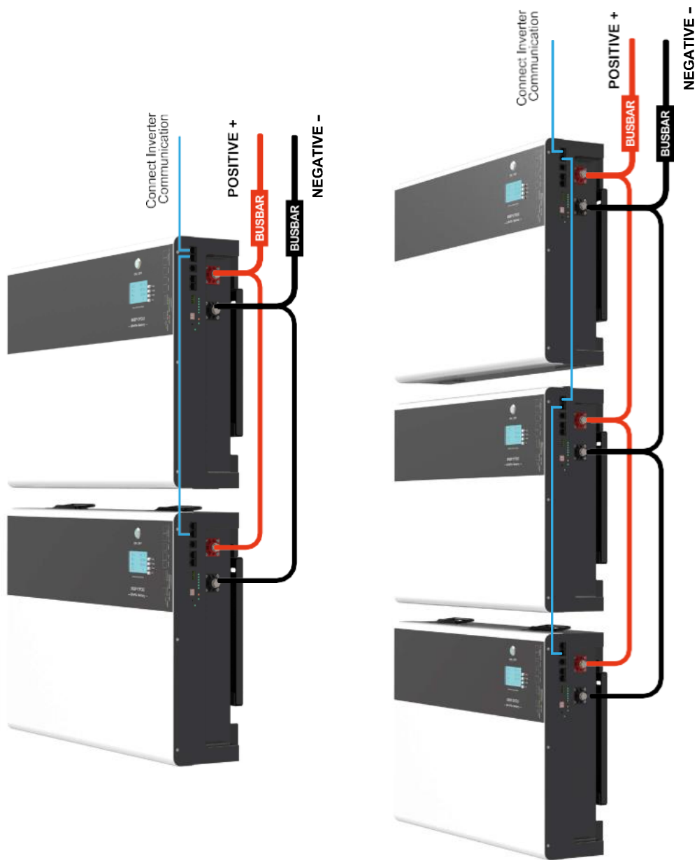
2 x Battery Parallel
